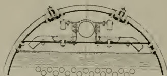
FEED PAN IN BOILER SHELL, ORLEANS RAILWAY.
